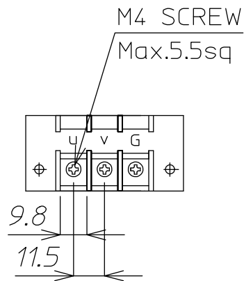
Output Terminal detailed chart
