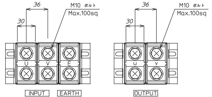
端子配列図 (TERMINAL ARRANGEMENT)
