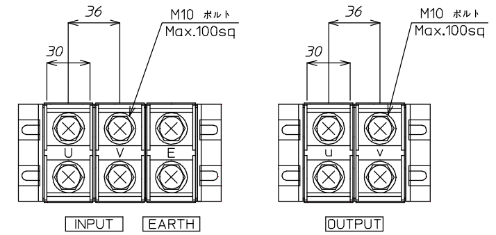
端子配列図 (TERMINAL ARRANGEMENT)
