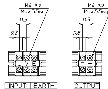
端子配列図 (TERMINAL ARRANGEMENT)
