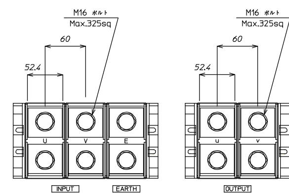
端子配列図 (TERMINAL ARRANGEMENT)
