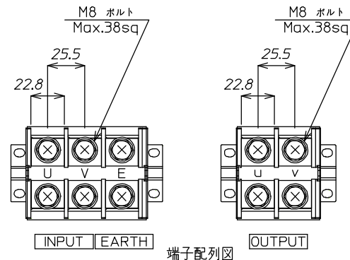
(TERMINAL ARRANGEMENT)
