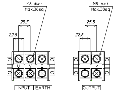
端子配列図 (TERMINAL ARRANGEMENT)
