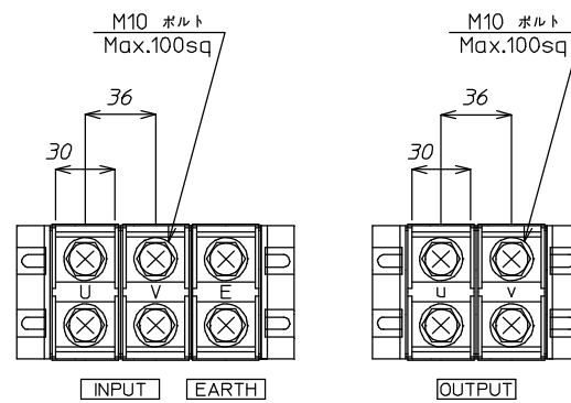
端子配列図 (TERMINAL ARRANGEMENT)
