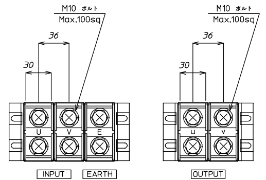
端子配列図 (TERMINAL ARRANGEMENT)
