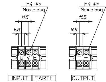
端子配列図 (TERMINAL ARRANGEMENT)
