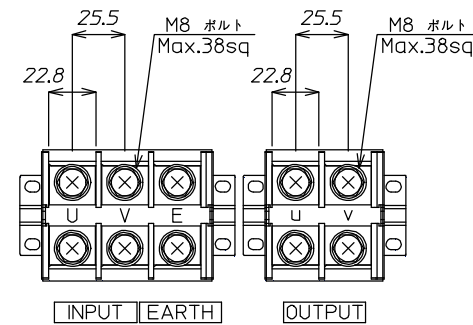
端子配列図 (TERMINAL ARRANGEMENT)
