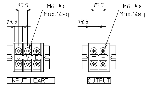
端子配列図 (TERMINAL ARRANGEMENT)
